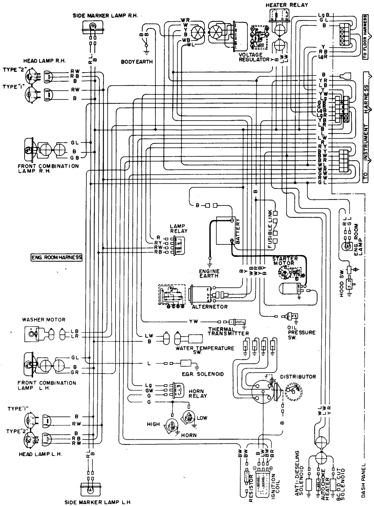
Fig. 10.36. Wiring diagram - 1974 USA - manual transmission
